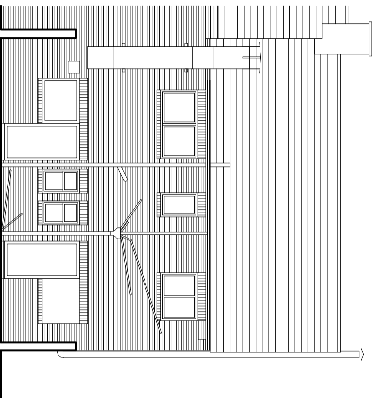
Existing South East Elevation
